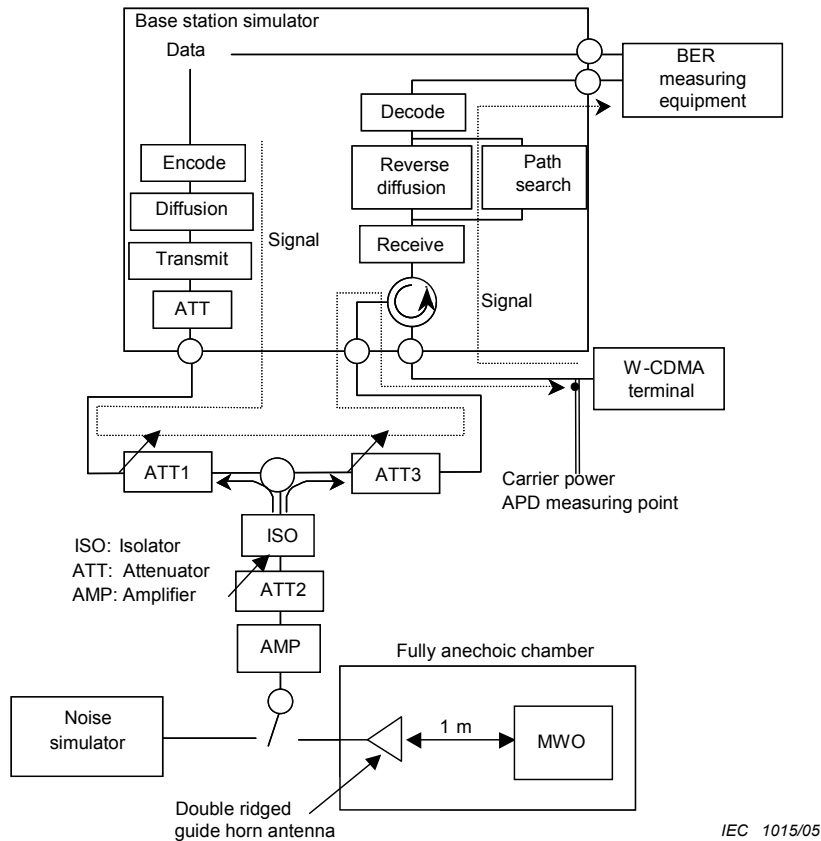
Figure 4.7.8 – Setup for measuring the BER of W-CDMA
