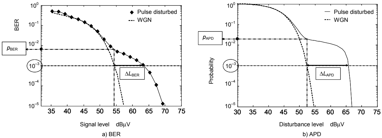
Figure 4.7.25 – Evaluation method of the correlation between BER and APD
