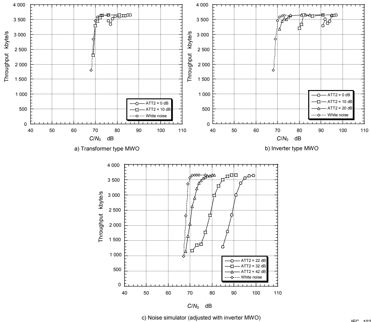
Figure 4.7.14 – PHS Throughput caused by radiation
