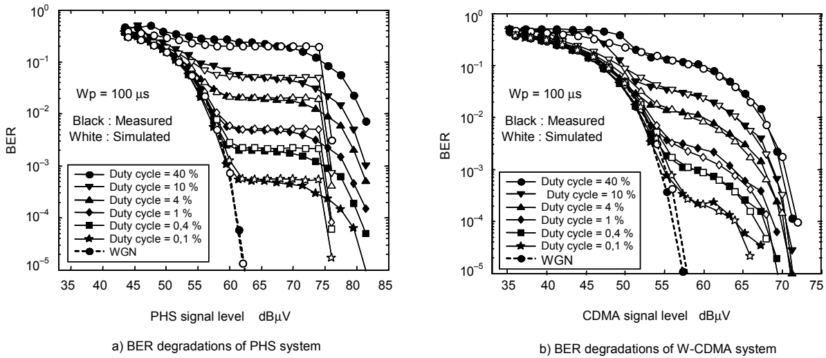
Figure 4.7.24 – BER degradation of PHS and W-CDMA caused by repetition pulse (Carrier power; –35 dBm)
