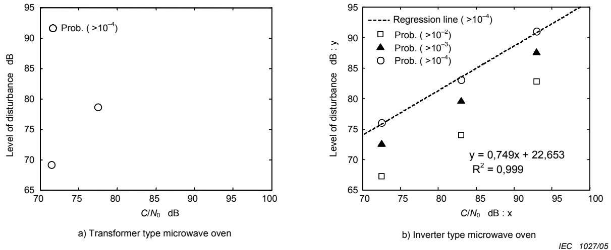
Figure 4.7.20 – Correlation of the disturbance voltages with the system performance( C/N_0 )
