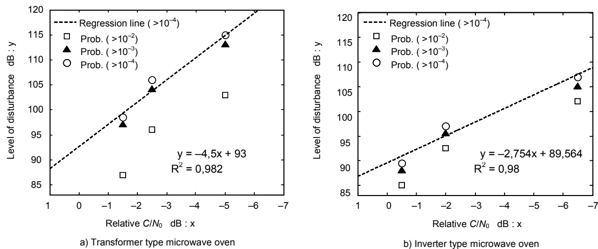
Figure 4.7.17 – Correlation of the disturbance voltages with the system performance
