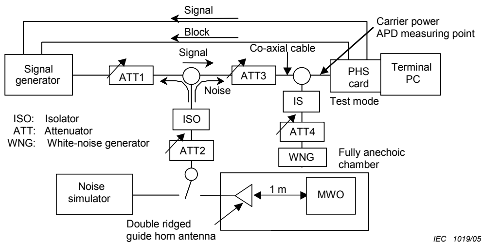
Figure 4.7.12 – Set-up for measuring the BER of PHS
