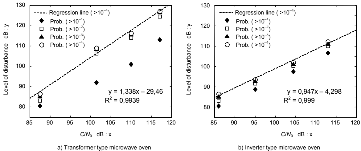
Figure 4.7.16 – Correlation of the disturbance voltages with the system performance( C/N_0 )
