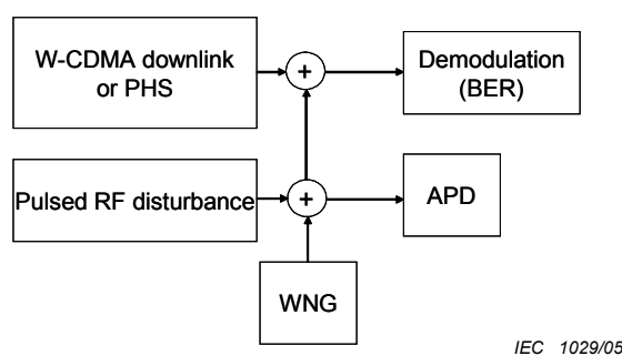
Figure 4.7.22 – Simulation set-up for estimating communication quality degradation of a PHS or W-CDMA
