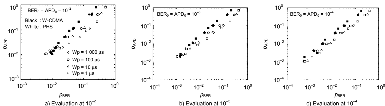
Figure 4.7.27 – Correlation between measured p_{BER} and p_{APD}
