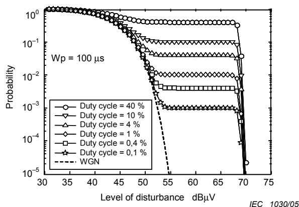
Figure 4.7.23 – APD of pulse disturbance
