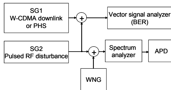
Figure 4.7.21 – Experimental set-up for measuring communication quality degradation of a PHS or W-CDMA
