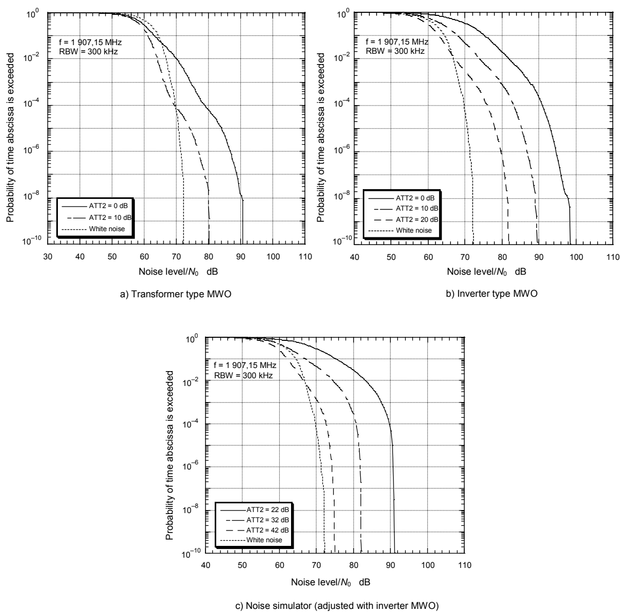
Figure 4.7.13 – APD characteristics of disturbance
