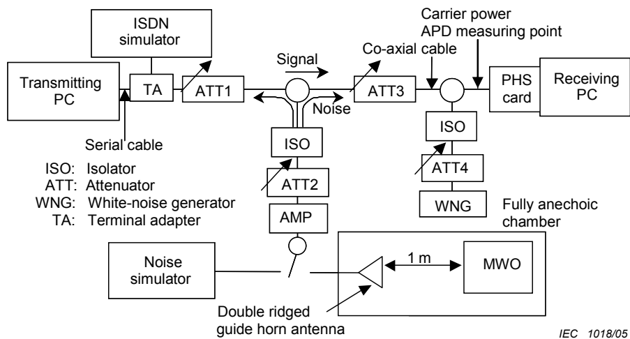
Figure 4.7.11 – Set-up for measuring the PHS throughput
