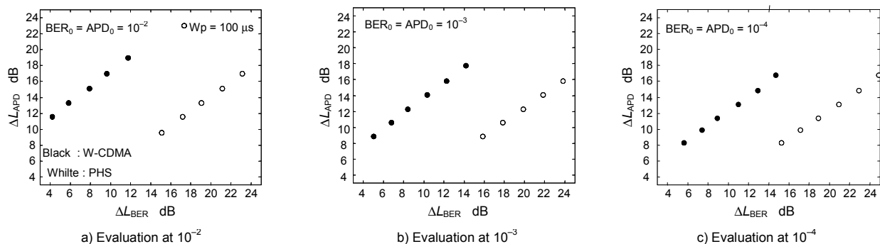
Figure 4.7.26 – Correlation between measured \Delta L_{BER} and \Delta L_{APD}
