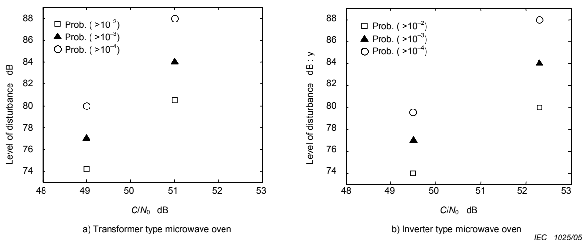
Figure 4.7.18 – Correlation of the disturbance voltages with the system performance
