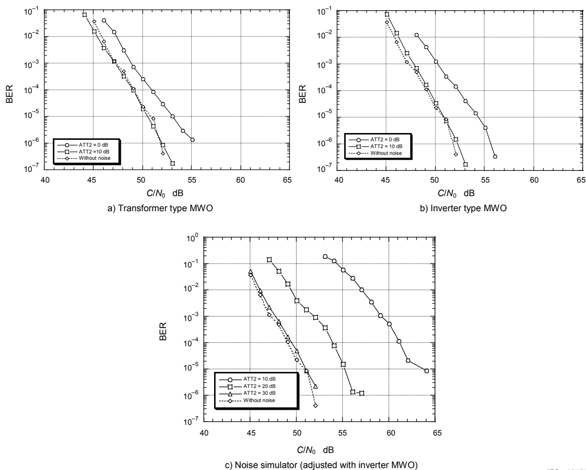
Figure 4.7.10 – BER of W-CDMA caused by radiation noise
