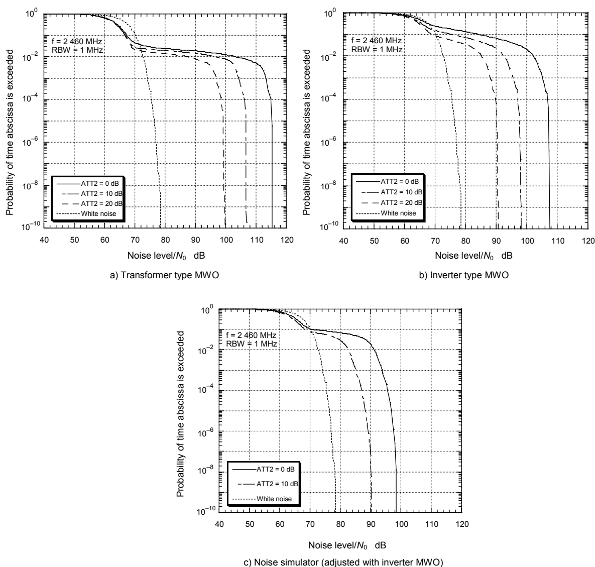
Figure 4.7.6 – APD characteristics of disturbance (2 460 MHz)
