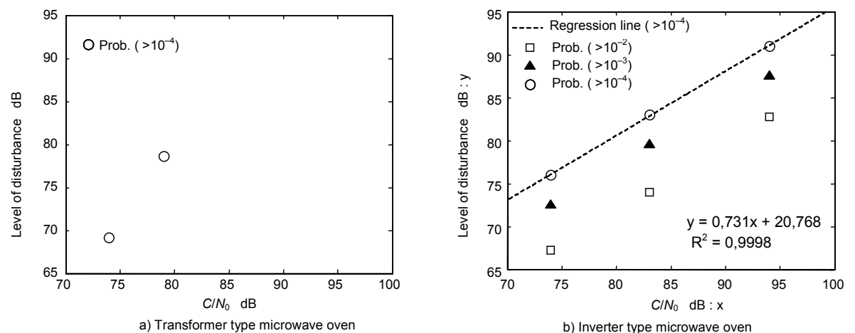
Figure 4.7.19 – Correlation of the disturbance voltages with the system performance( C/N_0 )
